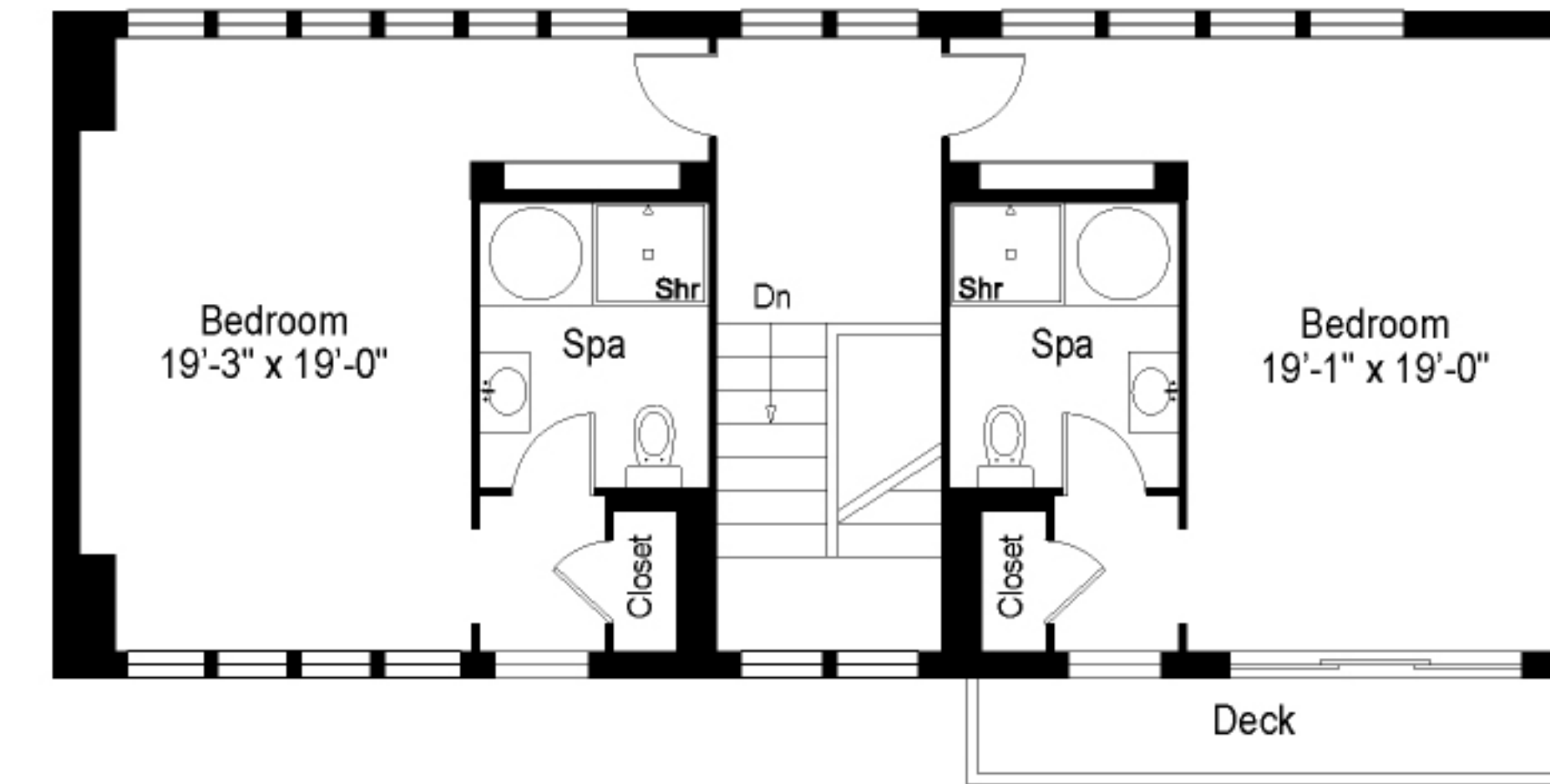
SECOND LEVEL NE-WING
