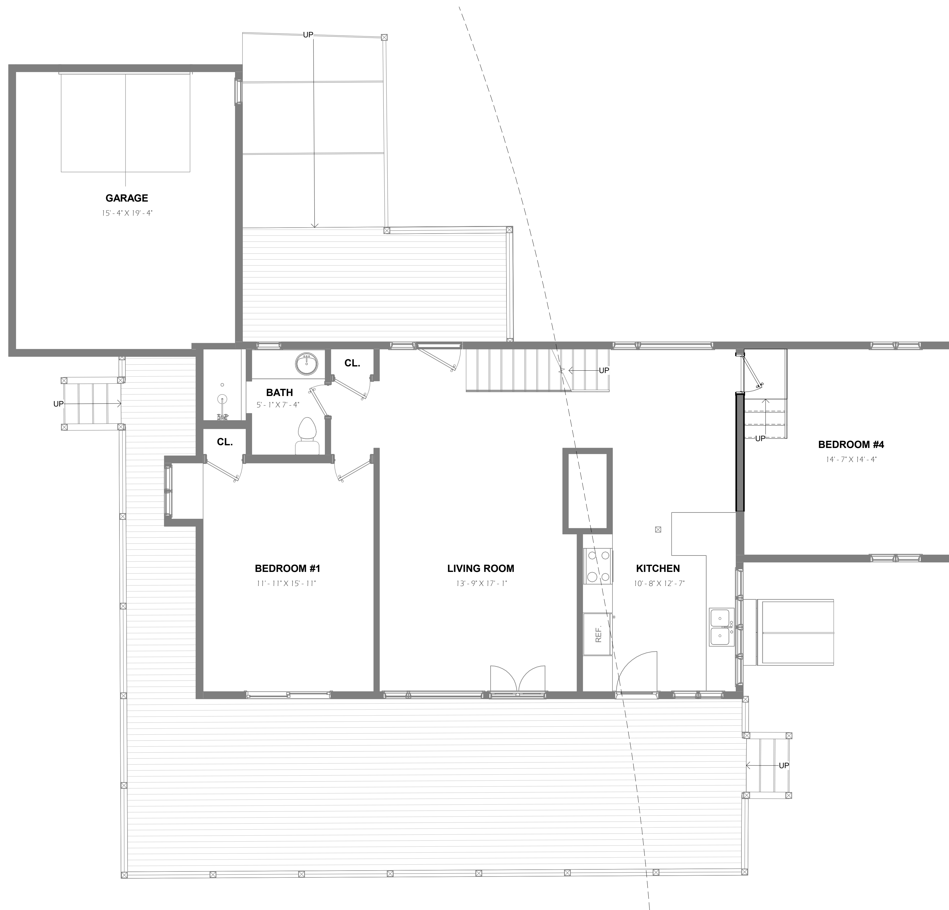
1 Proposed First Floor Plan - OPT. 3 1/4" = 1'-0"
